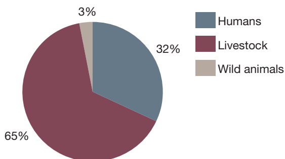
Figure 3. Global terrestrial vertebrate biomass
